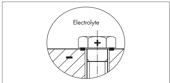
Contact corrosion
